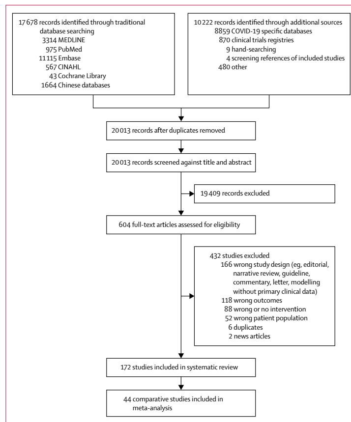
Figure 1: Study selection
